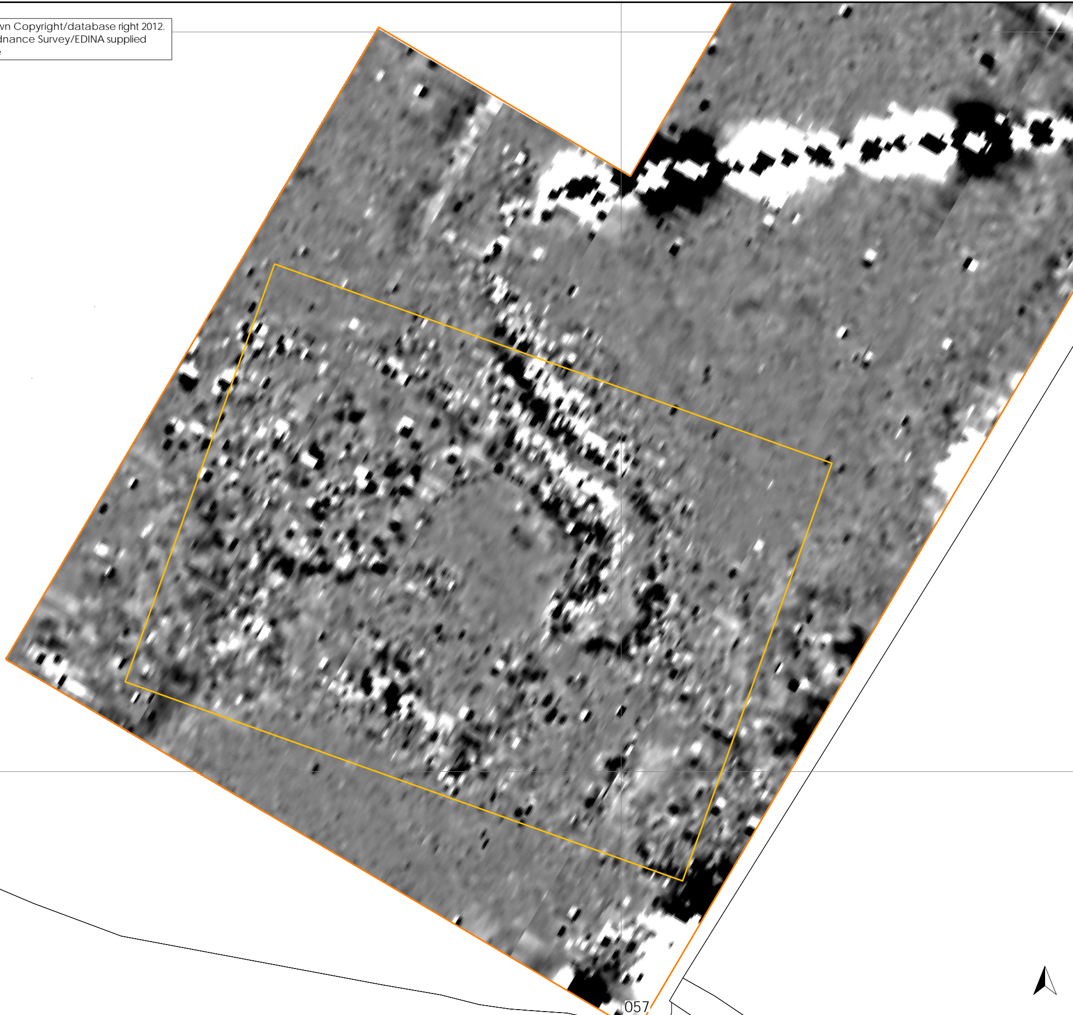
Figure 14: Cogden Hall extract from geomagnetic survey
