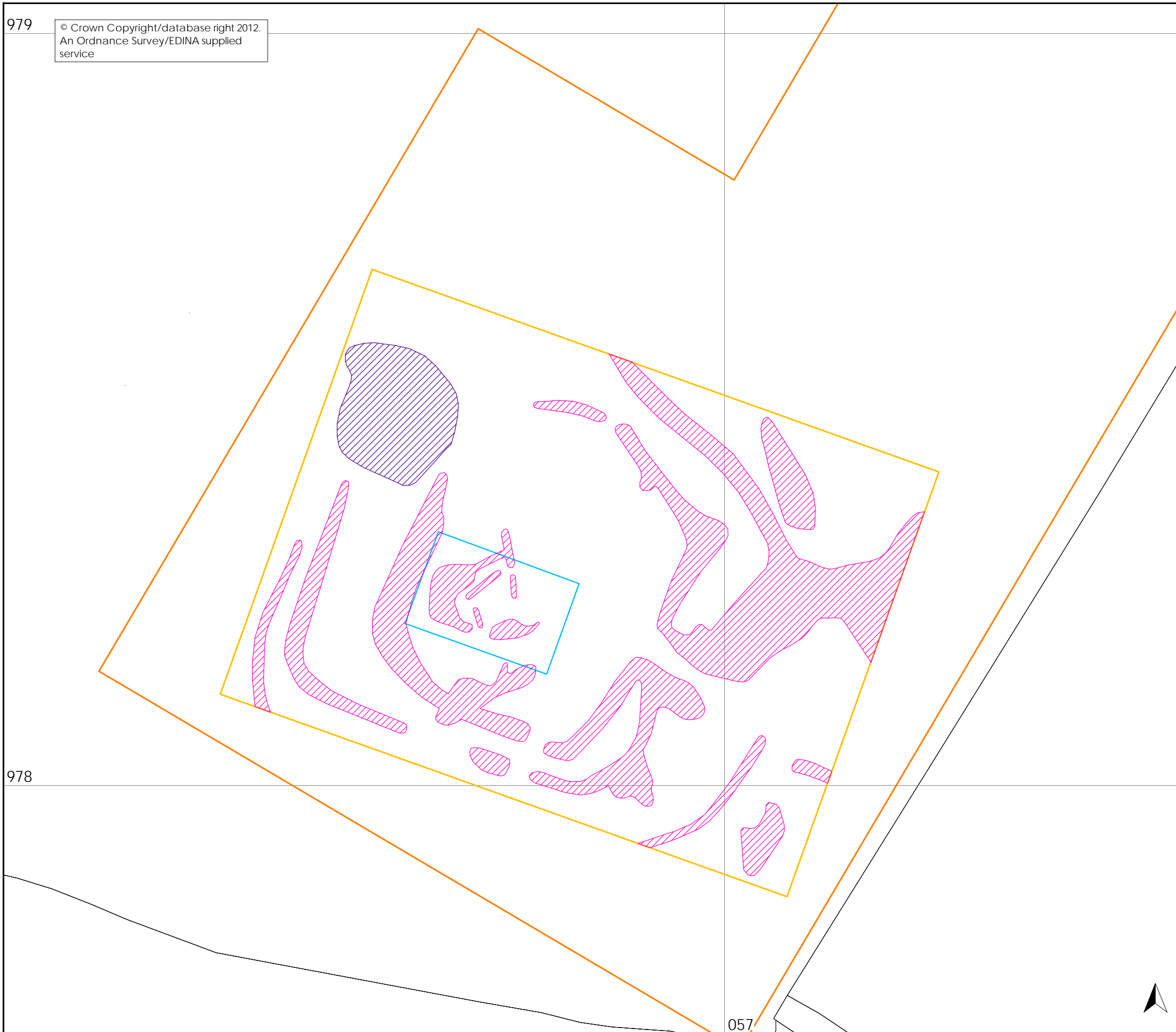
Figure 19: Cogden Hall geophysical interpretation of resistance data
